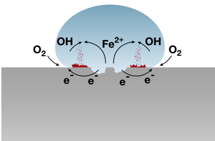
Fig. 3: Corrosion of iron under a drop of water, showing metal dissolution, oxygen reduction and the formation of rust.
