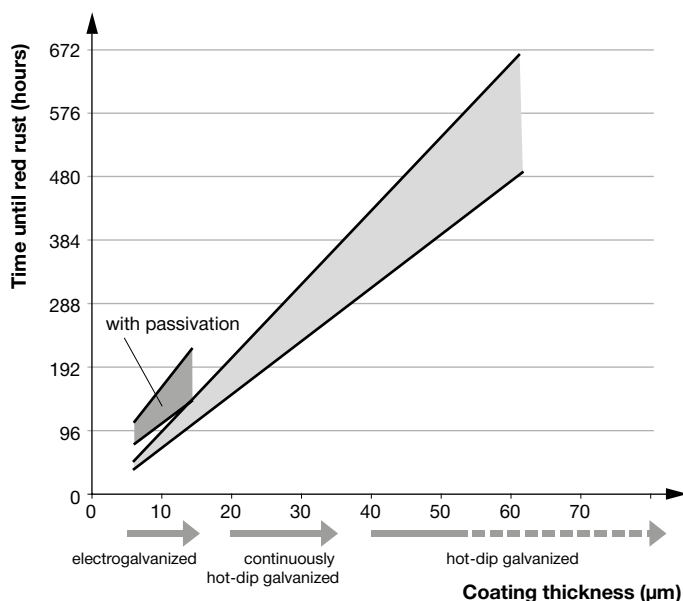
Fig. 15: Typical time until the first appearance of red rust (corrosion of the steel substrate) in the salt spray for zinc coated products with varying coating thickness.
