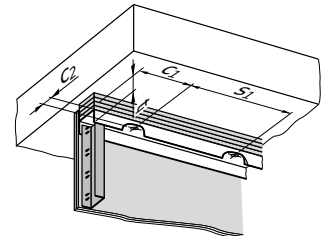
Deflection head track fastening with gypsum strips (optional with sealant)
