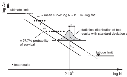
Statistical evaluation acc. to EN 1993-1-9 (EC 3)
