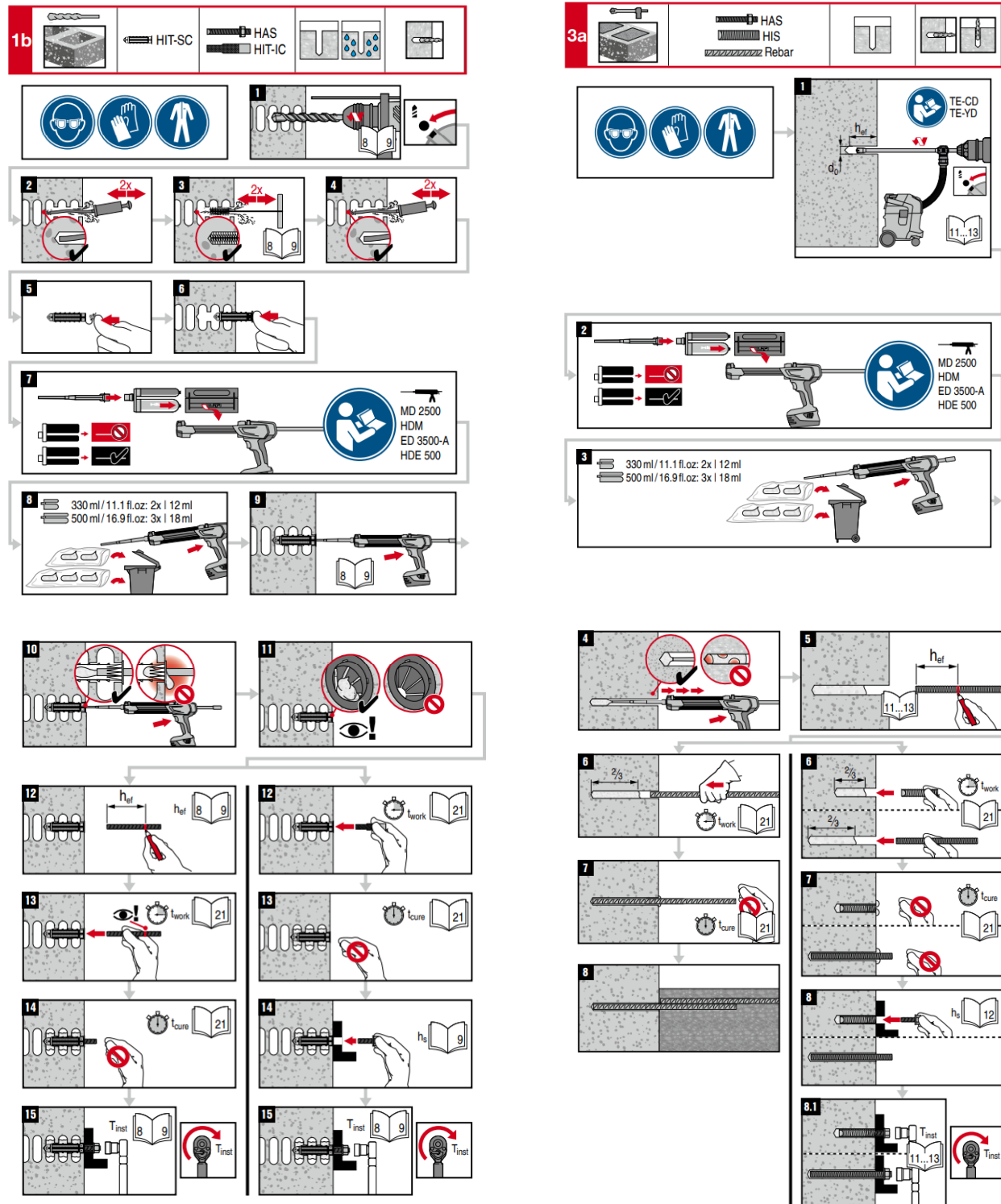
FIGURE 9—MANUFACTURERS PRINTED INSTALLATION INSTRUCTIONS (CONTINUED)
